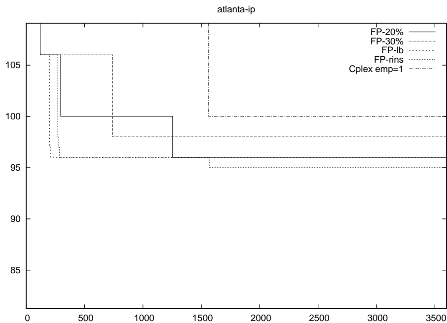
Figure 2: Incumbent solution over time (instance atlanta-ip)
