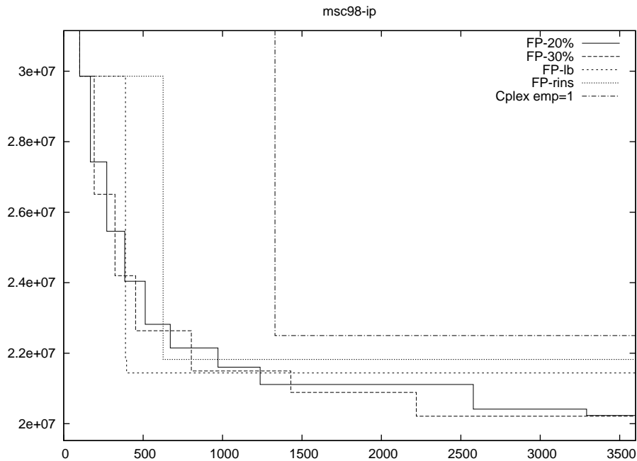
Figure 3: Incumbent solution over time (instance msc98-ip)
